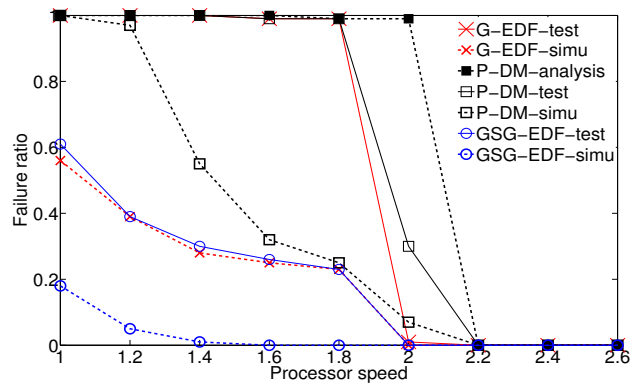
Fig. 6 Scheduling on a 40-core processor
