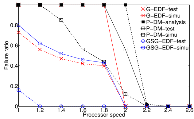
Fig. 7 Scheduling on an 80-core processor
