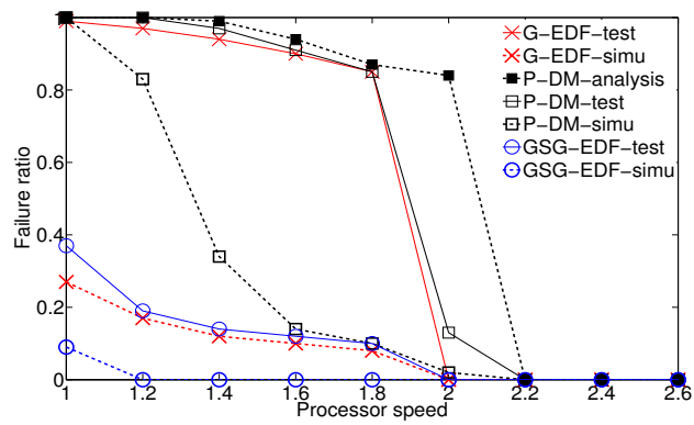
Fig. 5 Scheduling on a 20-core processor.
