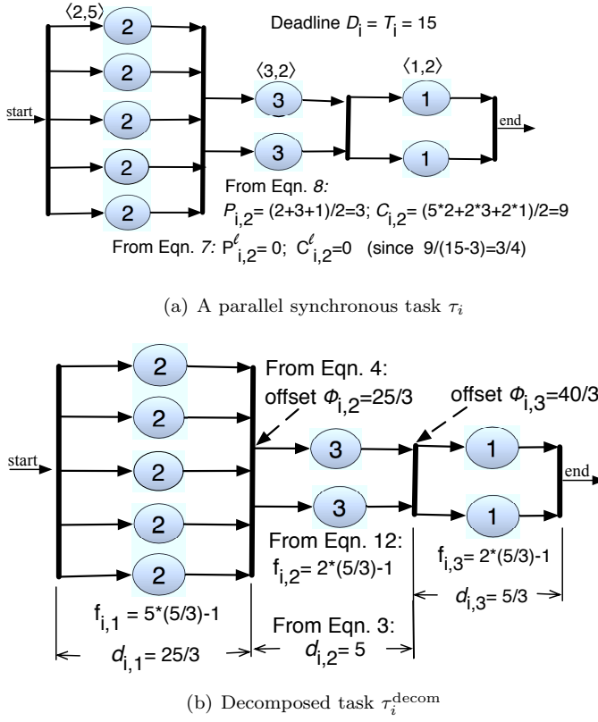
Fig. 3 An example of decomposition
